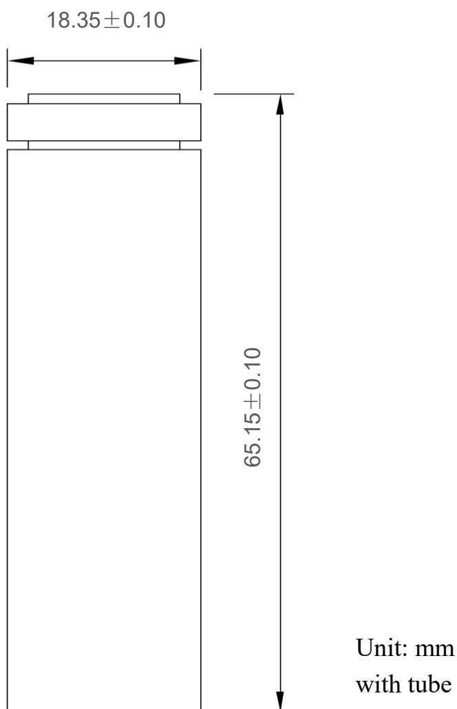
Fig. 1. Outline Dimensions of INR18650/30PL
